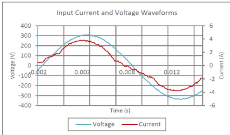
Input AC Current Waveform (ITHD = 14.19%, 50% Load)
